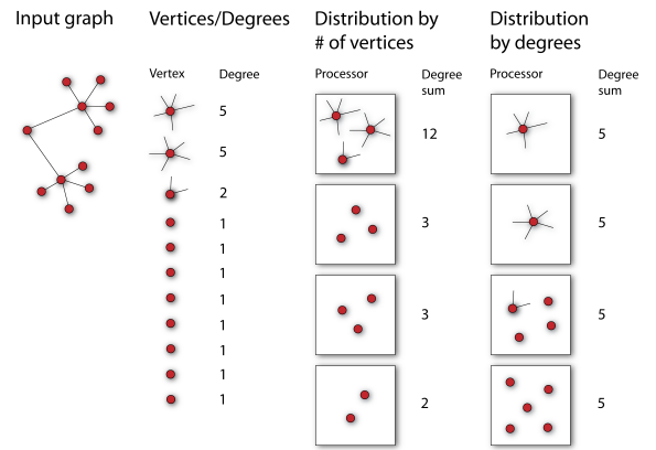
Figure 1: An illustrative example of two different vertex distribution strategies. The vertices ( n = 11 ) are represented as points, edges - as line segments, and processors ( p = 4 ) - as boxes. The first strategy shown is distribution that depends solely on the number of vertices. Each processor is assigned \lfloor \frac{n}{p} \rfloor vertices. The use of this strategy might result in one processor being assigned a large number of high degree vertices, thus having to conduct more inter-processor communication than other processors. The second strategy shown tries to alleviate this situation by taking into account vertex degrees. This strategy guarantees that the sums of degrees of the vertices assigned to each processor are approximately equal, thus providing a more balanced distribution.
