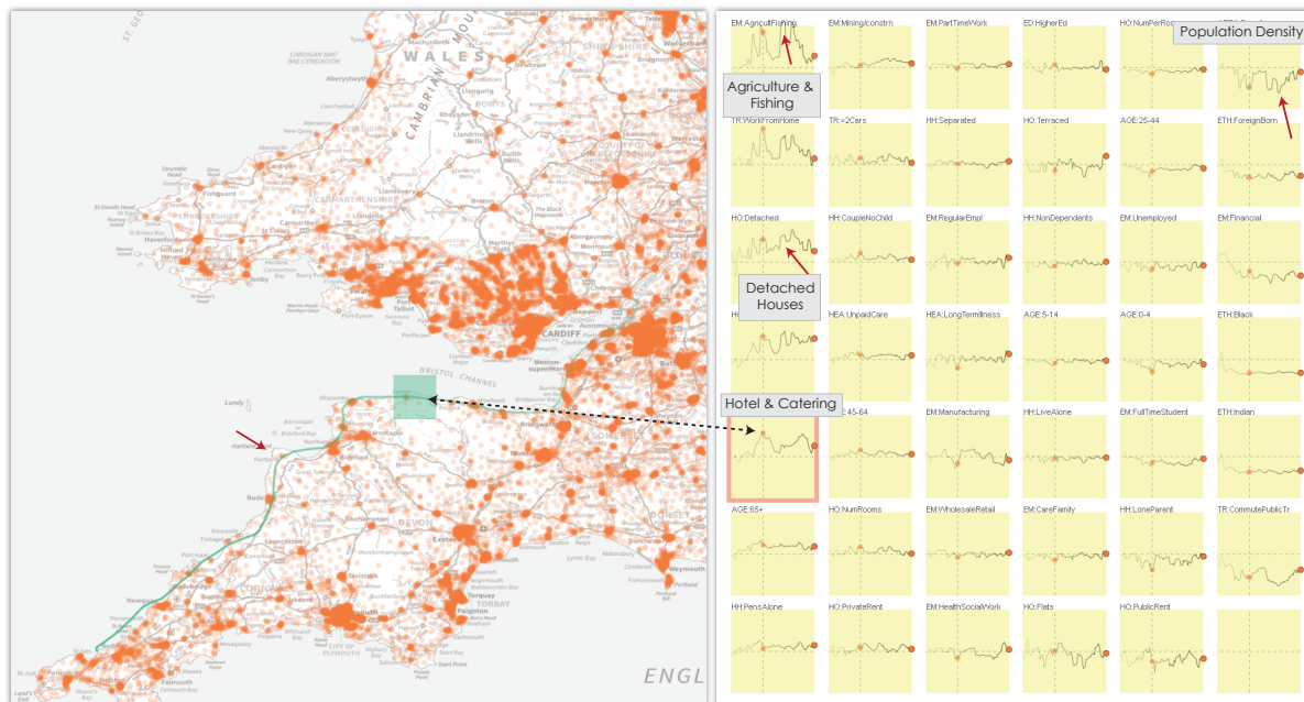
Fig. 1. Attribute signatures (right) are dynamically created in response to an interactive geographic selection sequence (left) that follows the coastline from South Gloucestershire to St Ives on the north Cornwall coast where each output area is represented with an orange dot. The signatures show how the average values for 41 attributes vary as the selection moves. The trace of the brush sequence is linked to the signatures – the faded points and the vertical dashed lines on the signatures are linked to the location highlighted on the map. A small holiday resort, Lynton (green rectangle), is characterized by the high proportion of population in the hotel and catering industry. Fishing & agriculture towns, such as Hartland (red markers), are characterized with low population densities where population is in mostly detached houses.
