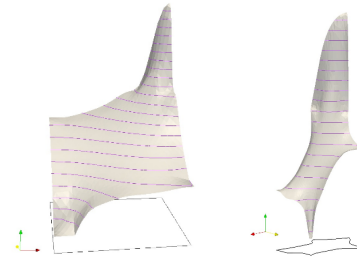
Figure 3: Left: Our computation of a monotonic surface inside the square [0, 1]^2 . Right: The same surface reparametrized inside the 2-cell. The purple lines are isovalues, they show that there is no critical points inside these surfaces.
