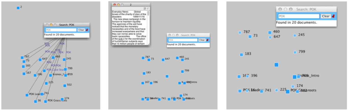
Fig. 6. Multi-model semantic interaction in StarSPIRE: Document relevance feedback. Left: The user explicitly searches for documents containing the term “POK.” Documents matching this search term are added to the display and arranged using a “near = similar” metaphor. Middle: The user selects the outlying document, opens it, then closes the document to remove it from the workspace. Right: The system decreases the entity weights of the terms contained in the deleted document. The system updates the visual encodings to reflect this relevancy feedback and updates the display layout.
