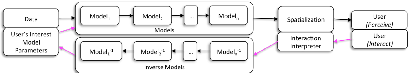
Fig. 3. Generalized multi-model semantic interaction visualization pipeline. Any number of models can be inserted for use in this pipeline. Once the user perceives the spatialization, they can choose to interact in it. This interaction feedback is interpreted as input to one or many inverted models. The updated model parameters are stored, which are then used, along with the original data, to create an updated spatialization.
