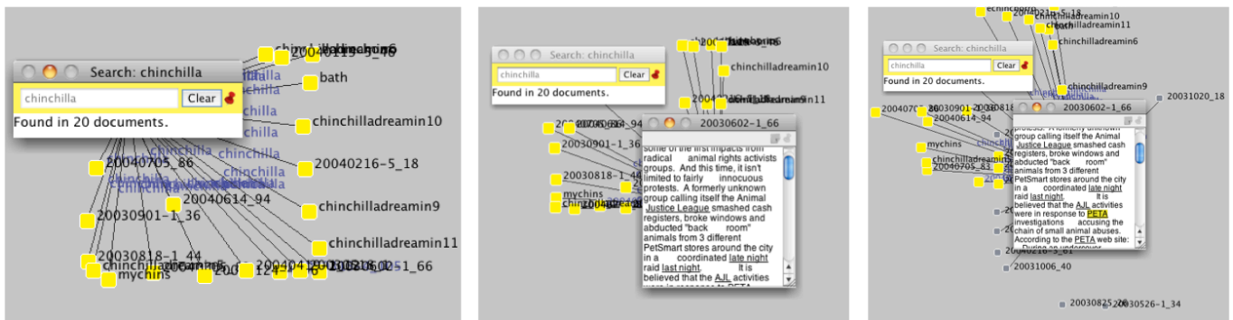
Fig. 7. Multi-model semantic interaction in StarSPIRE. Left: The user explicitly searches for documents containing the word “chinchilla.” Documents matching this search term are added to the display and arranged. Middle: The user selects a document to read. To prevent occlusion, nodes are pushed aside but still maintain their relationships to other documents as much as possible. Right: The user highlights the entity “PETA.” Eight new documents are retrieved and added to the display. Documents rearrange due to the shift in weighting scheme – documents that contain “chinchilla” and “PETA” (as well as other shared terms) are brought closer together in the middle, documents that contain only “chinchilla” are pushed to the top and left, and documents that only contain “PETA” are pushed to the bottom and right.
