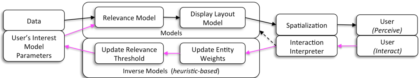
Fig. 4. Implemented version of the multi-model semantic interaction visualization pipeline. In StarSPIRE, a relevance model and a display layout model are used. With each user interaction, the perceived importance of terms updates, changing the spatial and the working set of data is modified. The dashed black arrow indicates typical force-directed layout interactions that do not influence the user’s interest model parameters.
