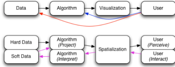
Fig. 2. Top: original visualization pipeline showing user interaction at the algorithmic and data levels Bottom: semantic interaction visualization pipeline showing user interaction within the spatialization, which is then interpreted by the model to extract parameters (stored in the system as “soft data”), which are used to update the spatialization.
