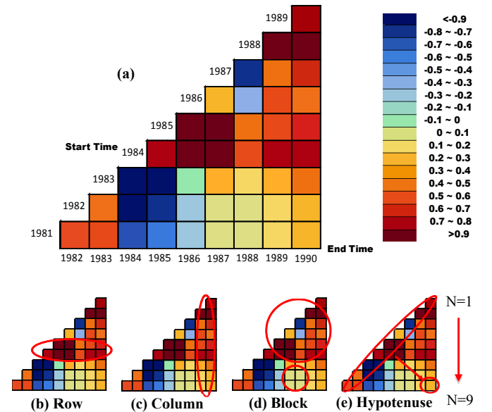
Fig. 6. A triangular component of Time Series Discs. (a) A yearly marked triangle. (b-e) Four important ways for reading the triangle.
