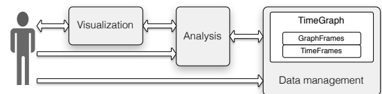
Figure 1: TimeGraph within the three layers of VA applications
