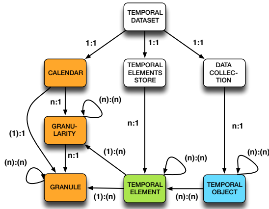
Figure 2: The TimeGraph data model for representing time-oriented information into a property graph structure: non-temporal aspects of data are modeled as properties of the TemporalObjects (cyan), temporal aspects are modeled as TemporalElements (green), while the graph substructure modelling the temporal reference system comprises Granule, Granularities, and Calendars (orange).
